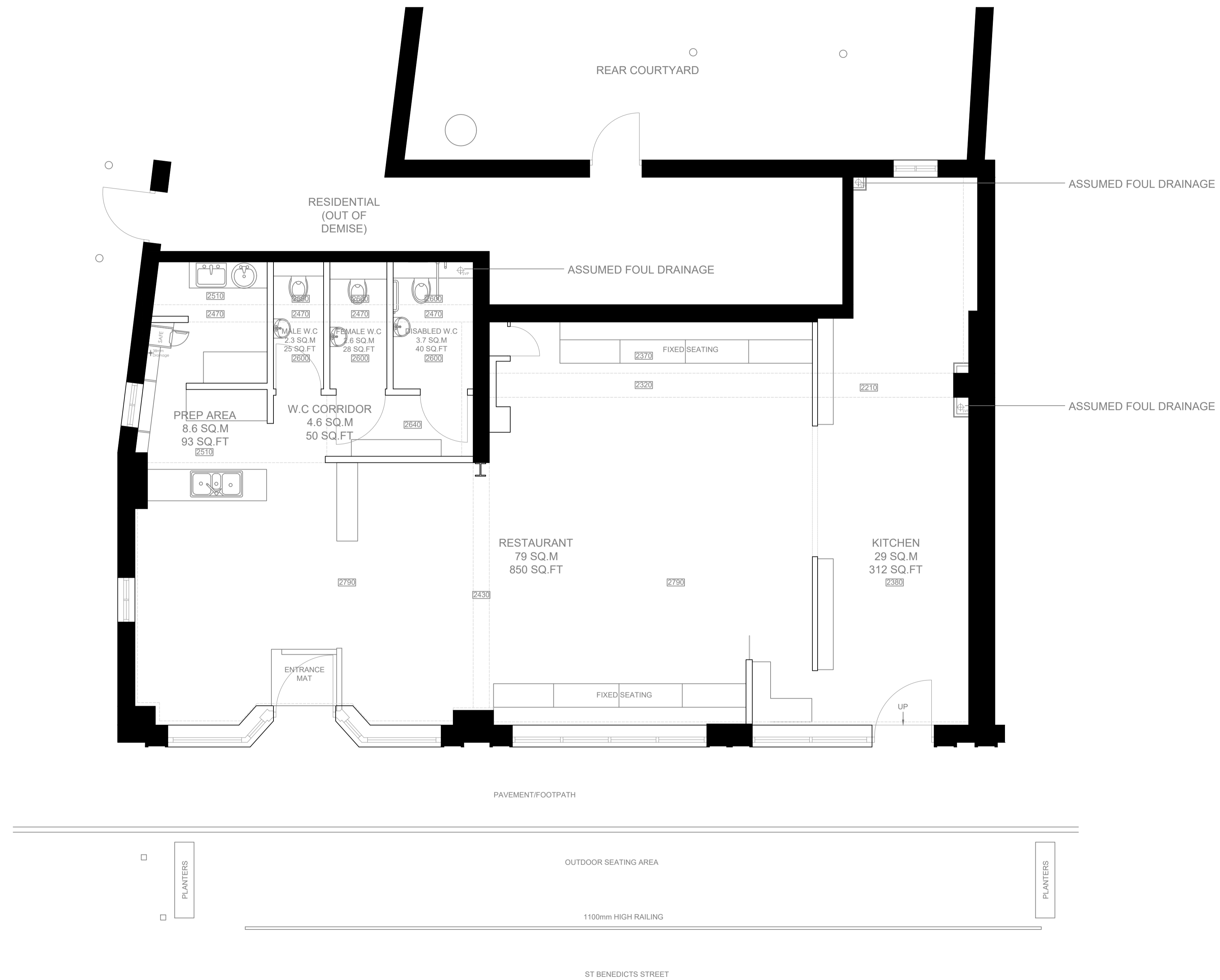
01 EXISTING GROUND FLOOR LAYOUT 1:50
